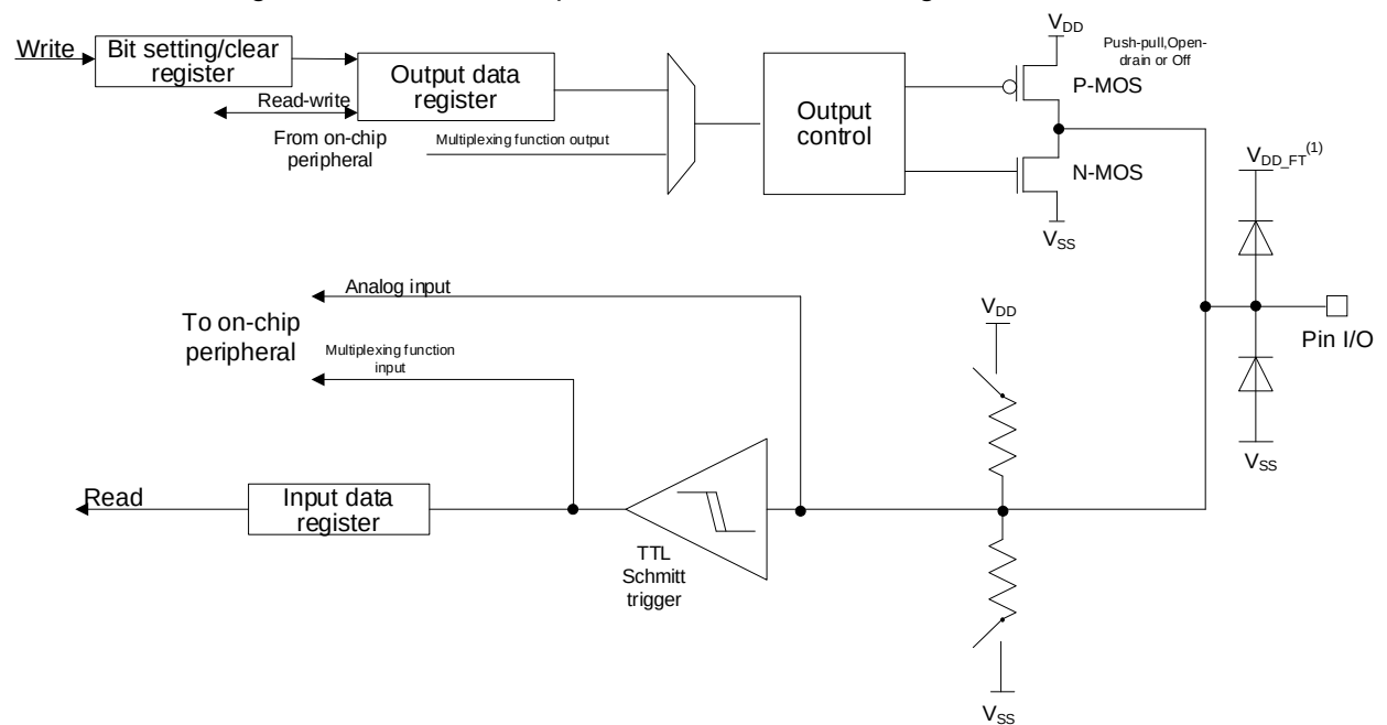
Figure 17 5V GPIO-compatible Structure Block Diagram
