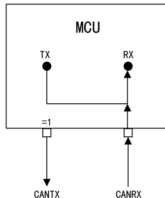
Figure 96 CAN Works in Silent Mode
