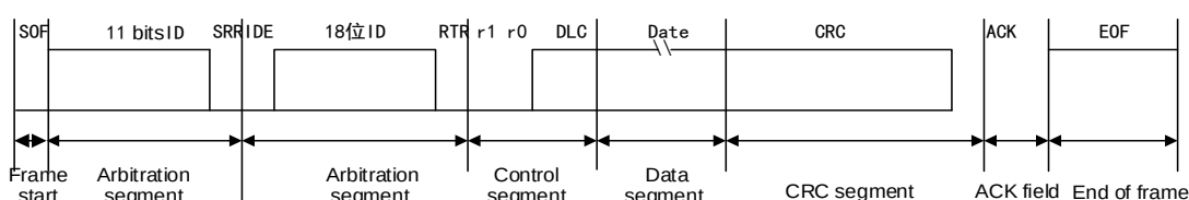
Figure 95 Extended Data Frame
