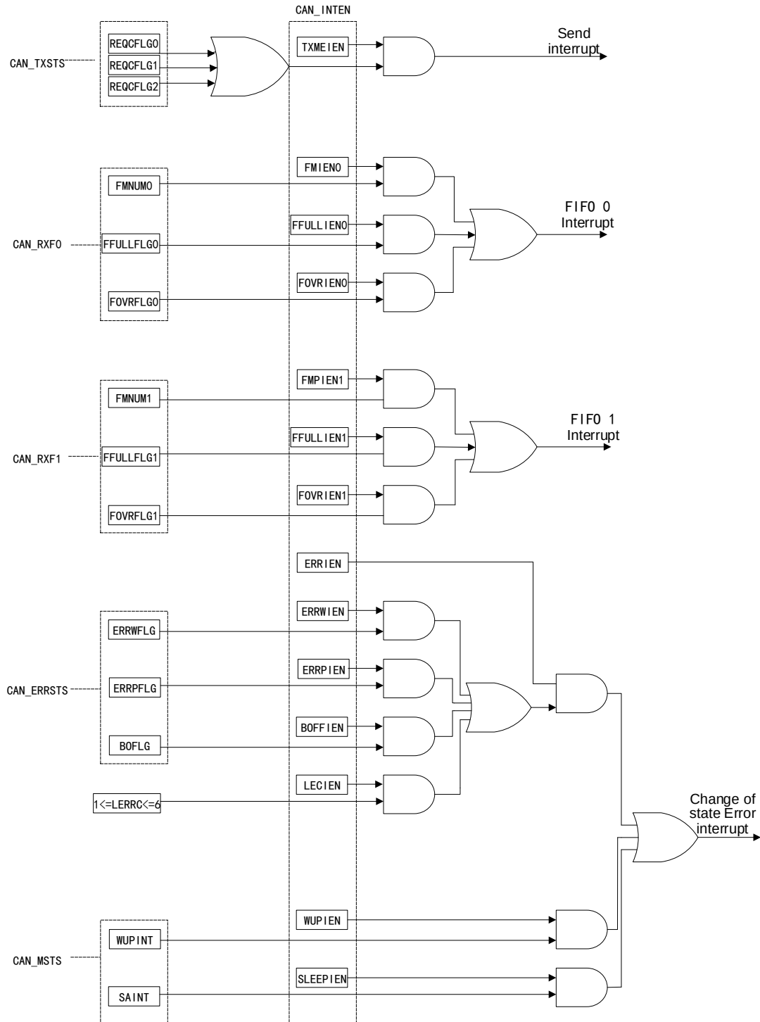
Figure 102 Event Flag and Interrupt Generation
