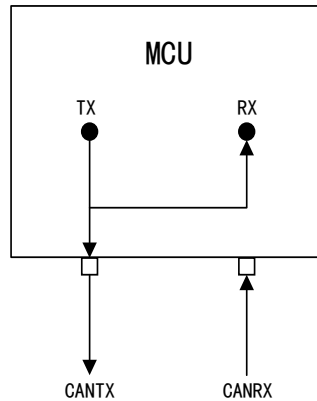
Figure 97 CAN Works in Loopback Mode
