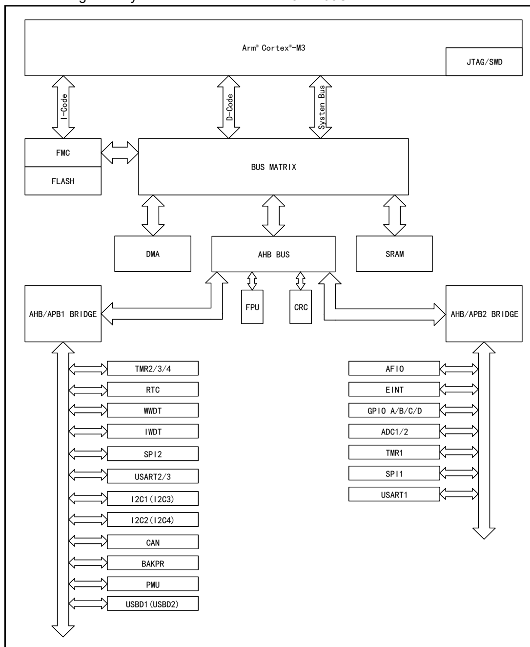
Figure 1 System Architecture of APM32A103CBT7 Series Products
