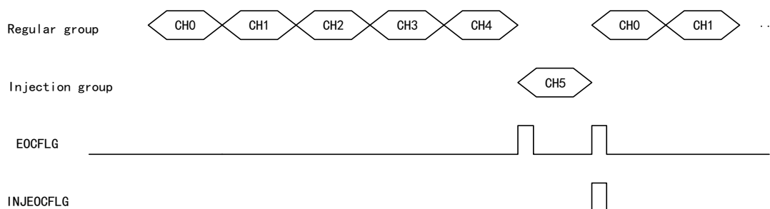
Figure 108 Automatic Injection Timing Diagram
