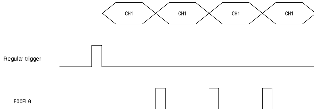
Figure 104 Continuous Conversion Mode Timing Diagram
