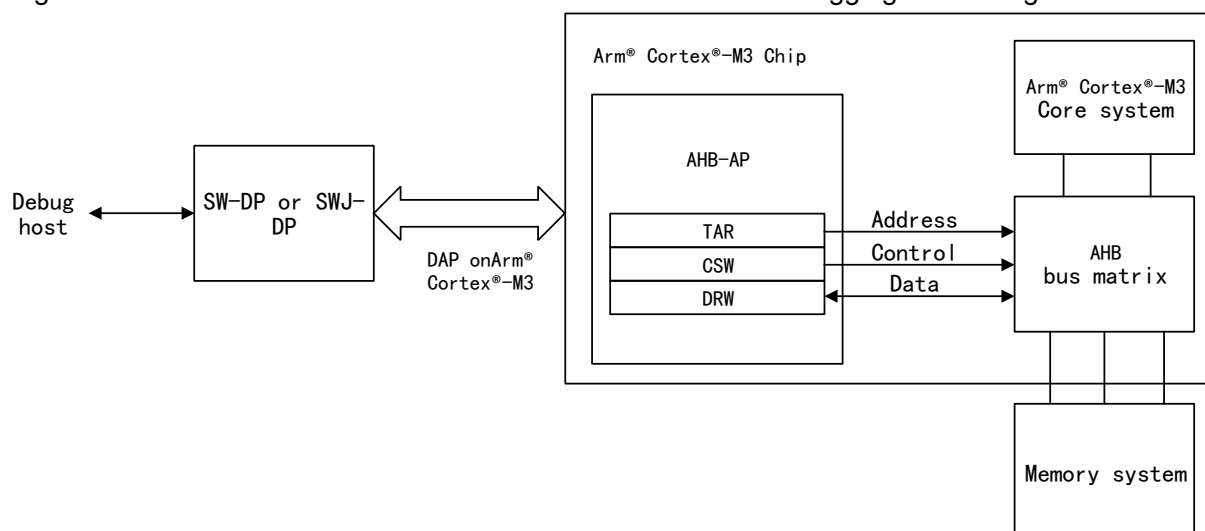
Figure 15 APM32A10xxx Level and Arm® Cortex® -M3 Level Debugging Block Diagram
