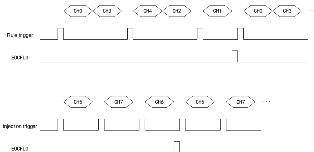
Figure 106 Discontinuous Mode Timing Diagram
