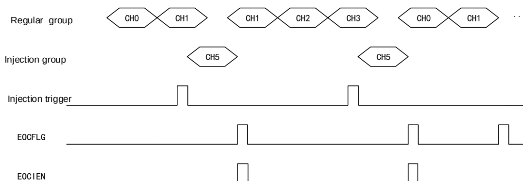
Figure 107 Trigger Injection Timing Diagram
