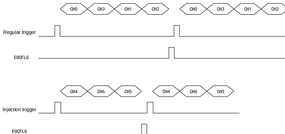
Figure 105 Scan Mode Timing Diagram
