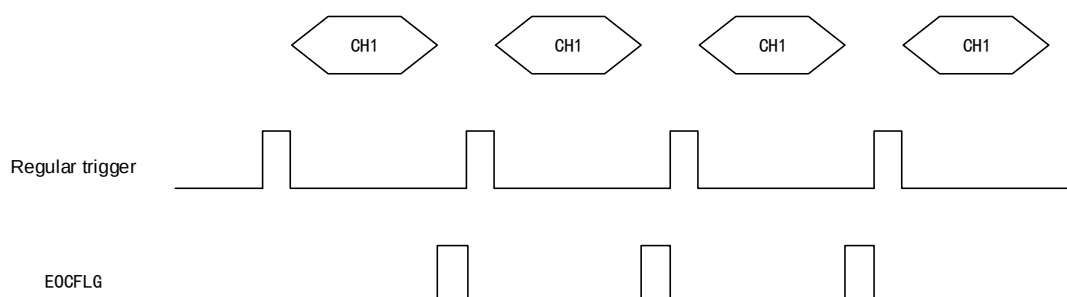
Figure 103 Single Conversion Mode Timing Diagram
