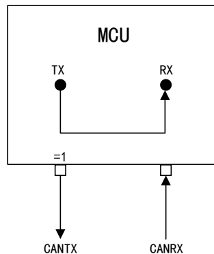
Figure 98 CAN Works in Silent Loopback Mode
